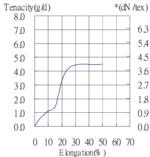
Typical Stress-strain Curve
